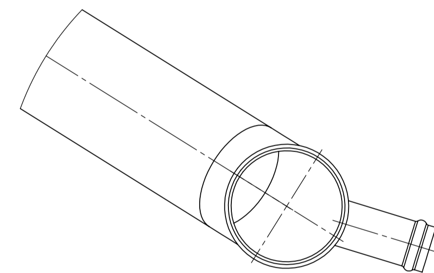
DETAIL B
